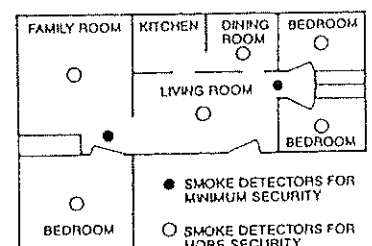
SMOKE DETECTOR LOCATIONS FOR SINGLE-FLOOR RESIDENCE WITH MORE THAN ONE SLEEPING AREA.
